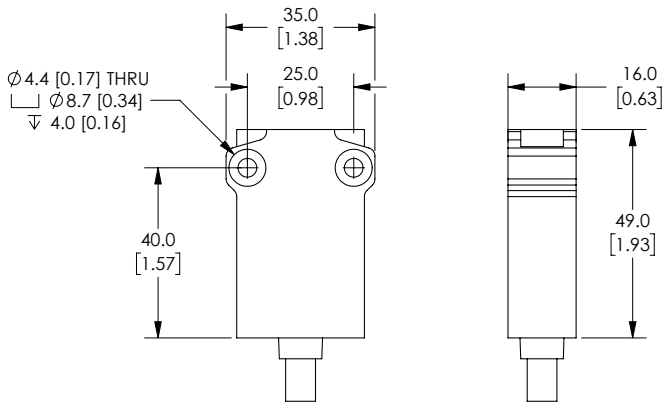
3.28 ft [1m] cable bottom exit
