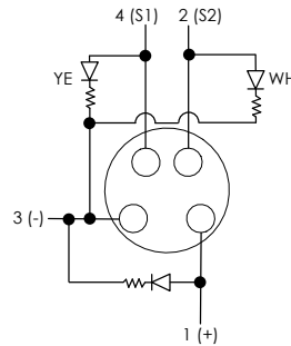
Diagram 4 (PNP field connection) 8000-84110-3580500 8000-88110-3950500 8000-84160-0000000
