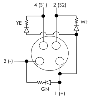
Diagram 6 (NPN field connection) 8000-84111-3580500 8000-88111-3950500
