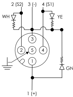
Diagram 1 (PNP field connection) 8000-84560-0000000 8000-88590-0000000
