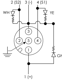
Diagram 2 (PNP field connection) 8000-88460-0000000
