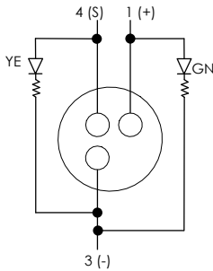
Diagram 3 (PNP field connection) 8000-84010-3370500 8000-88010-3570500 8000-84060-0000000 8000-88060-0000000
