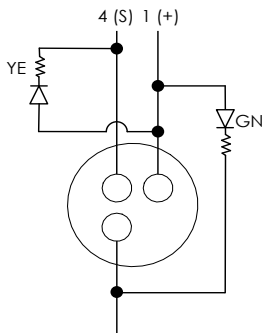
Diagram 5 (NPN field connection) 8000-84011-3370500 8000-88011-3570500
